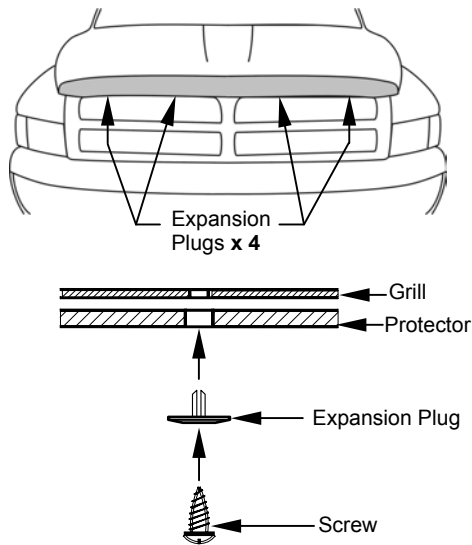
Illustration #1 : Protector Assembly
