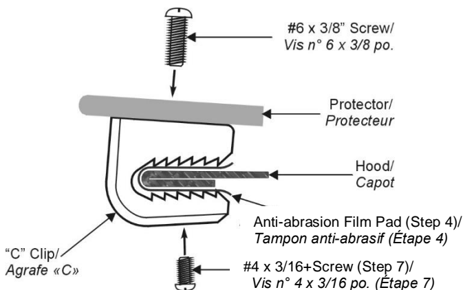
Illustration #1: CLIP CONFIGURATION/ Configuration de l'agrafe
