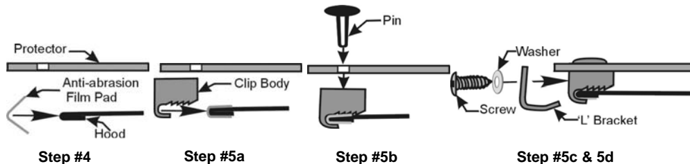
Illustration # 3: Clip Configuration - Patent No. 6,892,427
