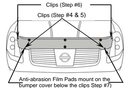
Illustration # 2: Clip Placement
